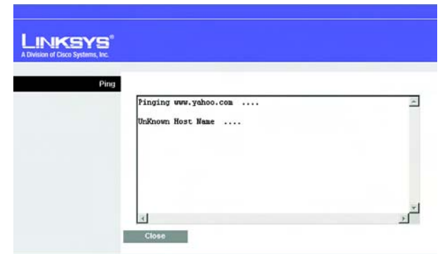
Figure 5-39: Ping Test
